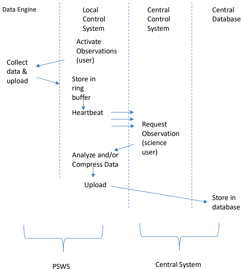
Figure 1342. Use Case 1. Request/Response process model.
