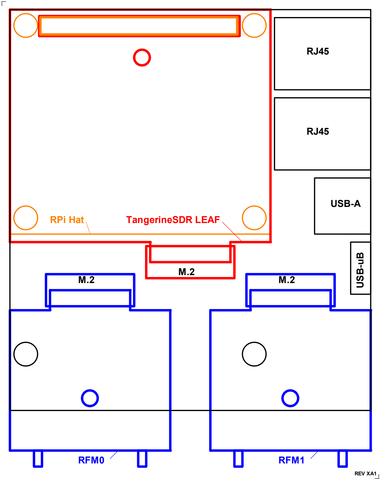
TangerineSDR Mechanical, Top View
